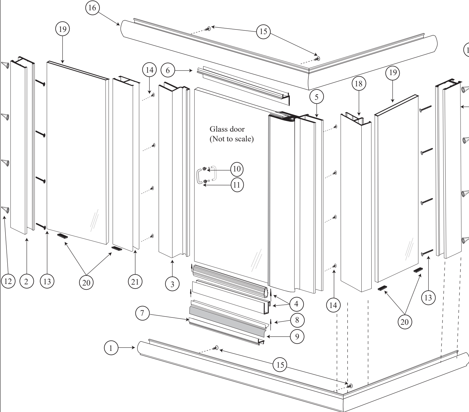
Detailed diagram of CH 1631 components
